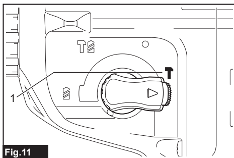
Fig.11 ► 1. Percussion uniquement
